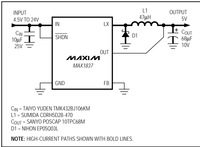
Figure 6. High-Voltage Application
