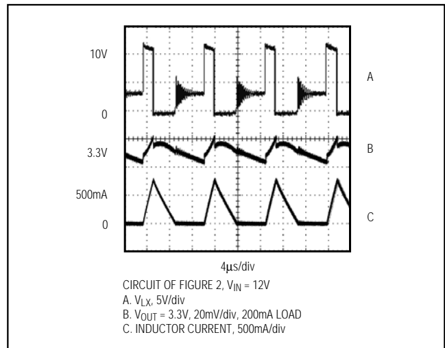
Figure 4. Discontinuous-Conduction Operation
